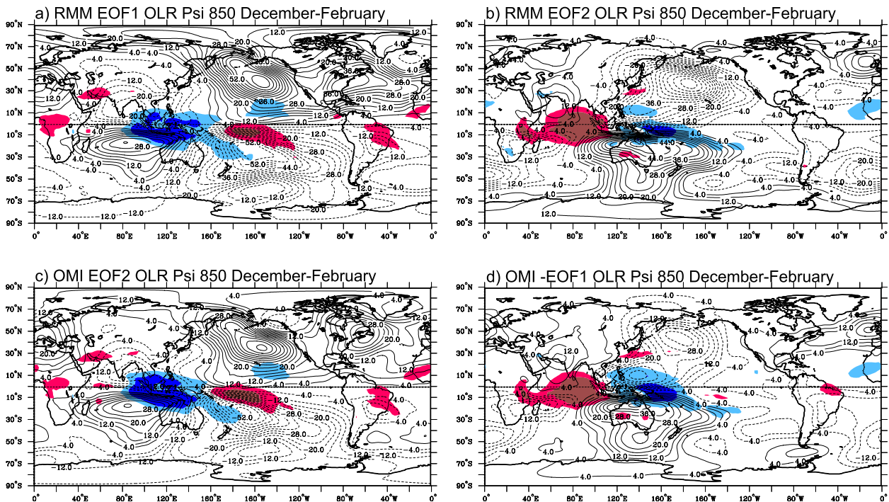
FIG. 3. Regressed OLR and 850-hPa streamfunction onto the daily December–February 1979–2012 PCs of (a) RMM EOF1, (b) RMM EOF2, (c) OMI EOF2, and (d) OMI -EOF1. All fields are scaled to a +2 standard deviation PC perturbation. OLR is shaded, starting at \pm 8 and 18 \text{ W m}^{-2} , with negative in blue. The streamfunction contour interval is 4 \times 10^5 \text{ m}^2 \text{ s}^{-1} .
