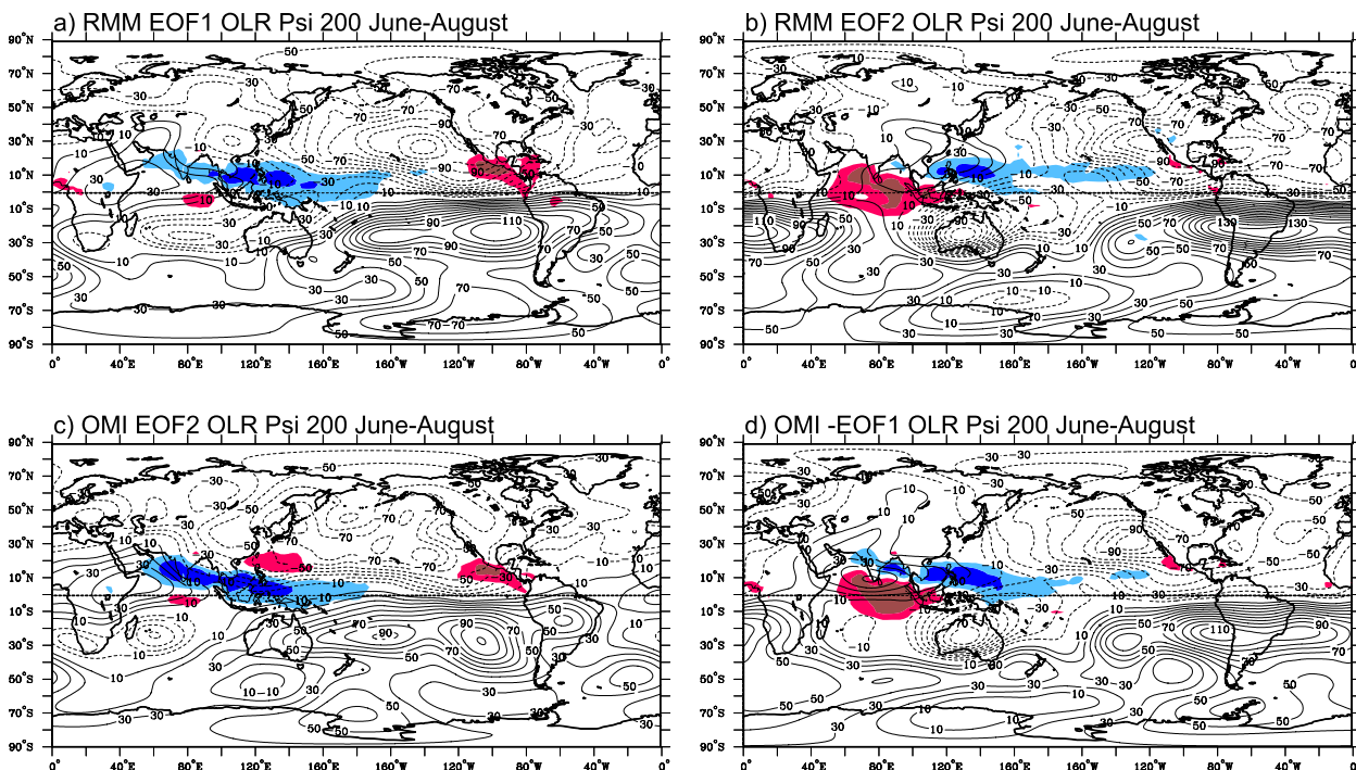
FIG. 4. As in Fig. 3, but for 200-hPa streamfunction during June–August 1979–2012 for (a) RMM EOF1, (b) RMM EOF2, (c) OMI EOF2, and (d) OMI-EOF1. The streamfunction contour interval is 10 \times 10^5 \text{ m}^2 \text{ s}^{-1} .
